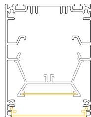
LTA70 B/H: 70x90 mm
