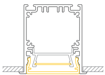
LTE50 B/H: 55 x 55 mm
