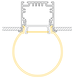
LTE40R B/H: 66 x 99 mm
