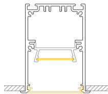
LTE57 B/H: 55 x 70 mm
