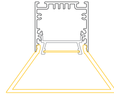
LTL40.T B/H: 80x73 mm
