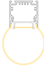
LTL40.R B/H: 66x99 mm
