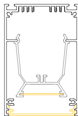
LTA60 B/H: 60x90 mm
