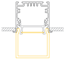
LTE40H B/H: 51 x 73 mm
