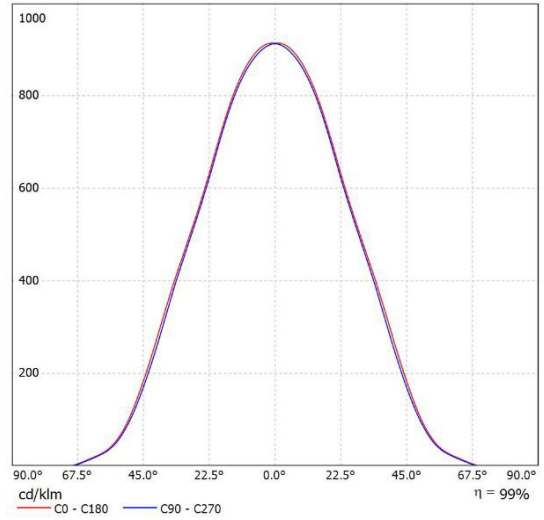
Leuchte: SML EL-E8R-30S-840 Lampen: 1 x SAMSUNG-4000K
