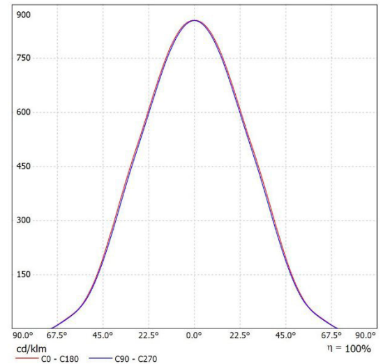
Leuchte: SML EL-E6R-20S-840 Lampen: 1 x SAMSUNG-4000K
