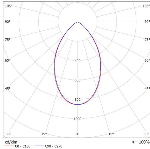
Leuchte: SML EL-E6R-20S-840 Lampen: 1 x SAMSUNG-4000K
