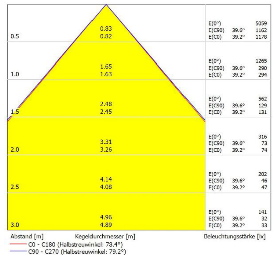
Leuchte: SML EL-E8F-20S-840 Lampen: 1 x SAMSUNG-4000K
