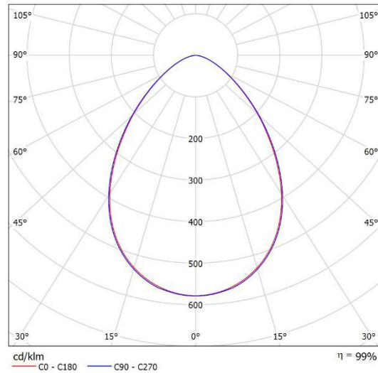
Leuchte: SML EL-E8F-20S-840 Lampen: 1 x SAMSUNG-4000K
