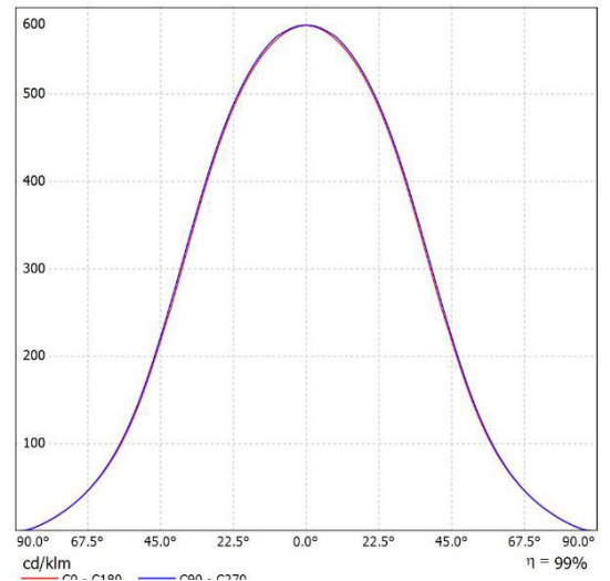
Leuchte: SML EL-E8F-20S-840 Lampen: 1 x SAMSUNG-4000K
