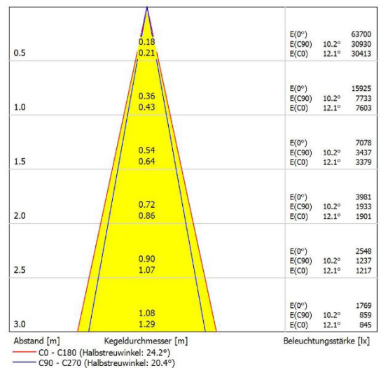
Leuchte: SML EL-BETA-A-C3-940-18 Lampen: 1 x CITIZEN-4000K
