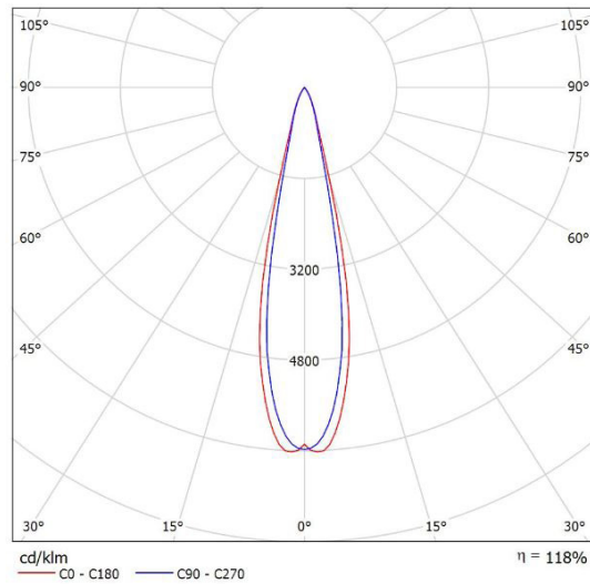
Leuchte: SML EL-BETA-A-C3-930-18 Lampen: 1 x CITIZEN-3000K
