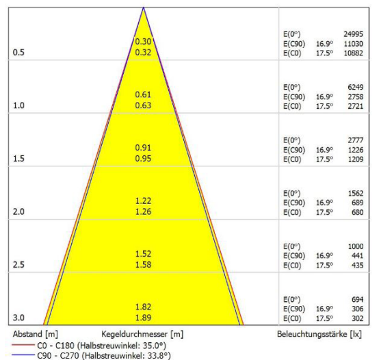
Leuchte: SML EL-BETA-A-C3-830-35 Lampen: 1 x CITIZEN-3000K
