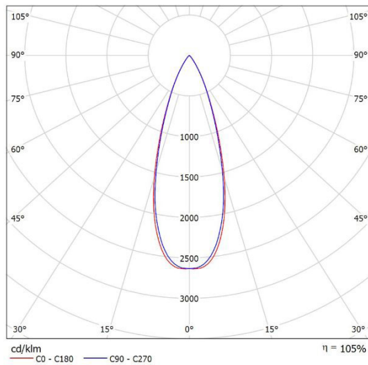
Leuchte: SML EL-BETA-A-C3-830-35 Lampen: 1 x CITIZEN-3000K
