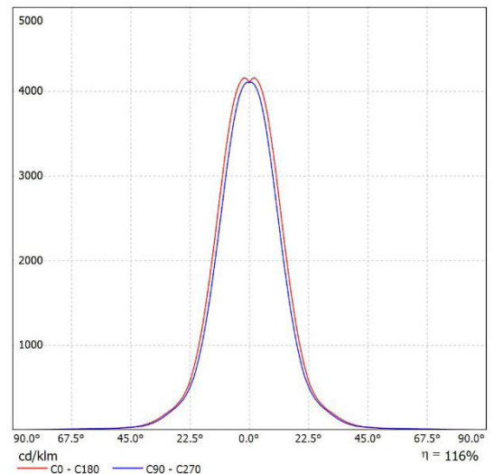
Leuchte: SML EL-BETA-C3-930-25 Lampen: 1 x CITIZEN-3000K
