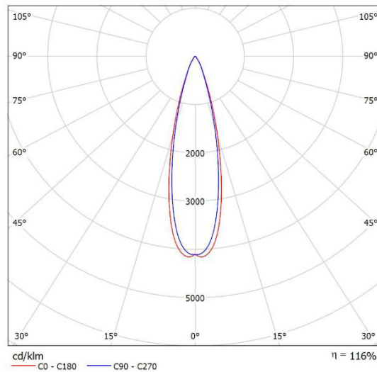
Leuchte: SML EL-BETA-C3-930-25 Lampen: 1 x CITIZEN-3000K
