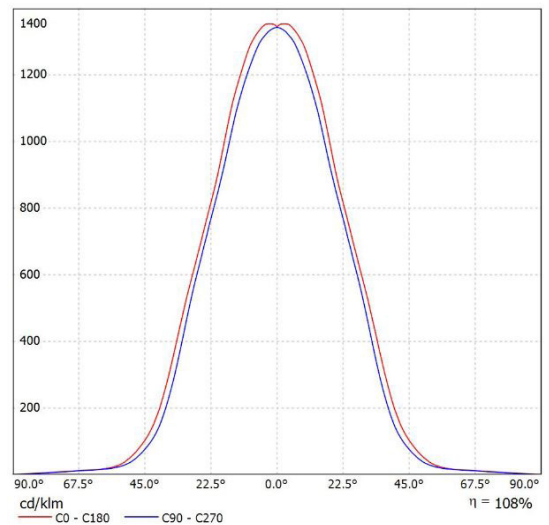
Leuchte: SML EL-BETA-C3-840-50 Lampen: 1 x CITIZEN-4000K
