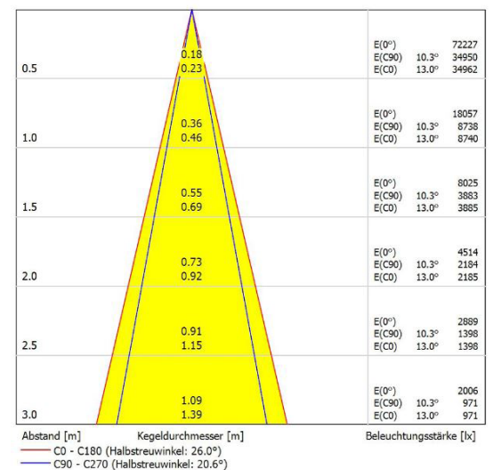
Leuchte: SML EL-BETA-C3-840-18 Lampen: 1 x CITIZEN-4000K
