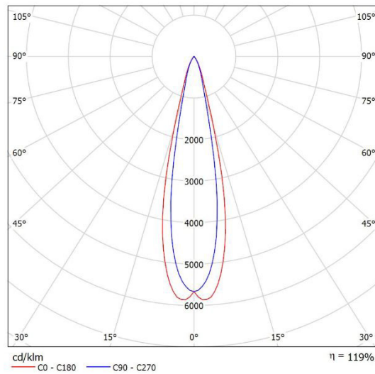
Leuchte: SML EL-BETA-C3-840-18 Lampen: 1 x CITIZEN-4000K
