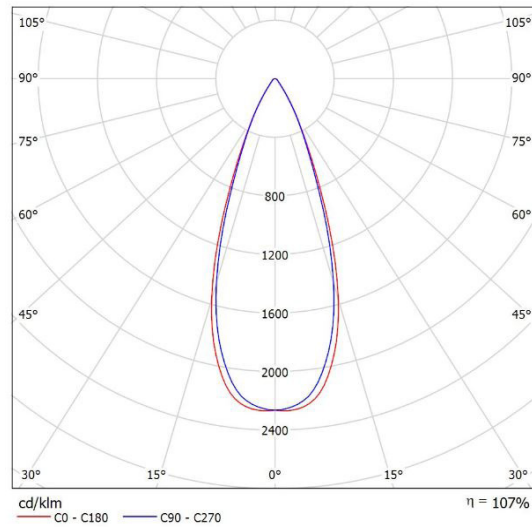
Leuchte: SML EL-BETA-C3-830-35 Lampen: 1 x CITIZEN-3000K
