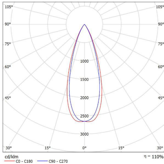
Leuchte: SML EL-ALPHA M-A-30T-940-35 Lampen: 1 x CITIZEN-4000K
