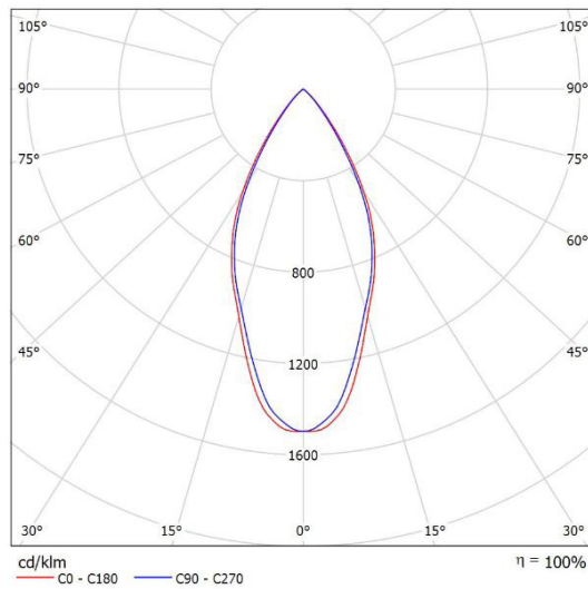
Leuchte: SML EL-ALPHA M-A-30T-930-50 Lampen: 1 x CITIZEN-3000K
