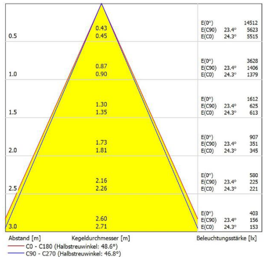
Leuchte: SML EL-ALPHA M-A-30T-930-50 Lampen: 1 x CITIZEN-3000K
