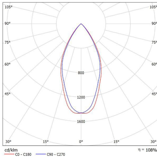
Leuchte: SML EL-ALPHA M-A-30T-840-50 Lampen: 1 x CITIZEN-4000K
