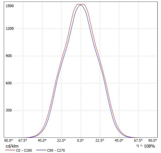
Leuchte: SML EL-ALPHA M-A-30T-840-50 Lampen: 1 x CITIZEN-4000K
