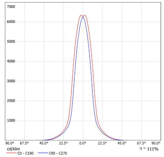
Leuchte: SML EL-ALPHA M-A-30T-840-18 Lampen: 1 x CITIZEN-4000K
