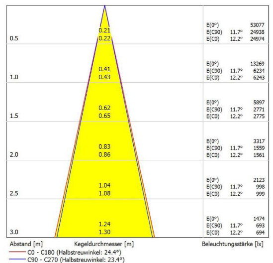
Leuchte: SML EL-ALPHA M-A-30T-830-25 Lampen: 1 x CITIZEN-3000K
