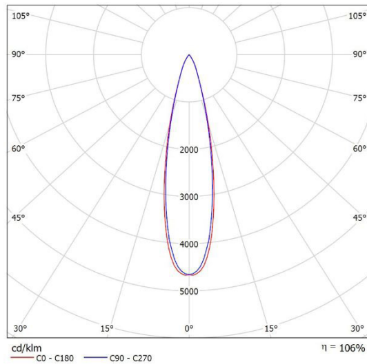
Leuchte: SML EL-ALPHA M-A-30T-830-25 Lampen: 1 x CITIZEN-3000K
