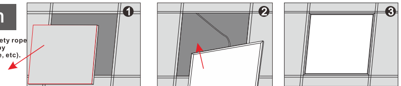
1. Remove the plasterboard from the ceiling. 2. Fix the panel into ceiling. 3. Installation finished.
