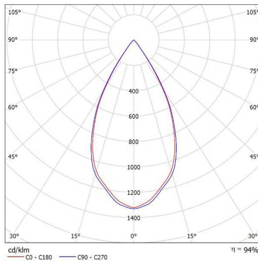
Leuchte: SML EL-T6-30T-840-55D Lampen: 1 x CITIZEN-4000K
