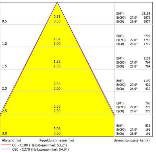
Leuchte: SML EL-T6-30T-840-55D Lampen: 1 x CITIZEN-4000K
