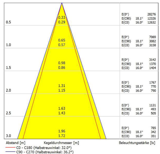
Leuchte: SML EL-T6-30T-830-35D Lampen: 1 x CITIZEN-3000K
