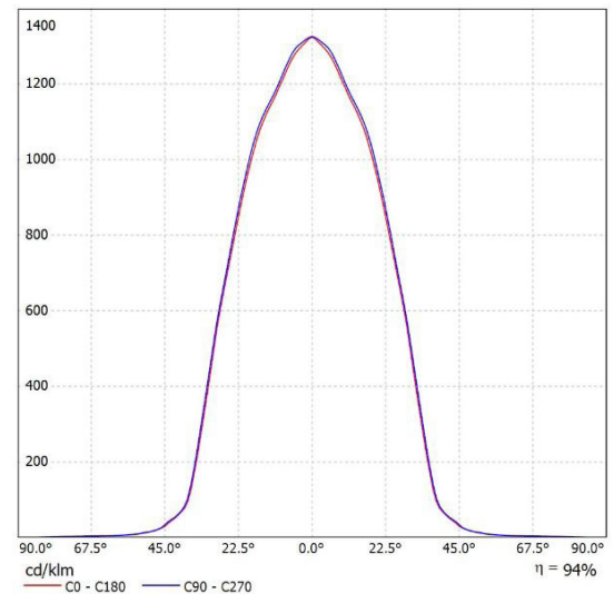
Leuchte: SML EL-T6-20T-840-55D Lampen: 1 x CITIZEN-4000K
