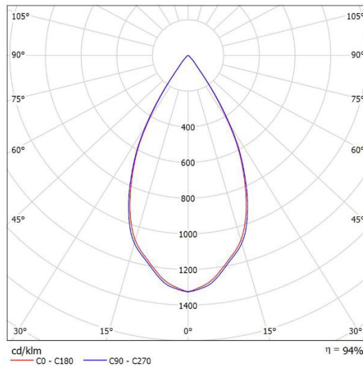
Leuchte: SML EL-T6-20T-840-55D Lampen: 1 x CITIZEN-4000K
