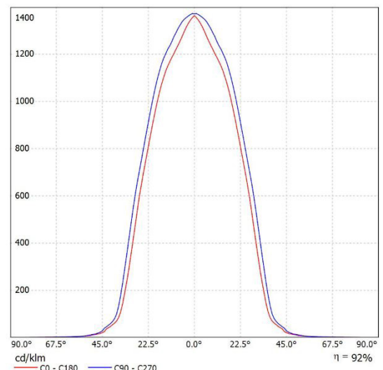
Leuchte: SML L-T6-20T-830-55D Lampen: 1 x CITIZEN-3000K
