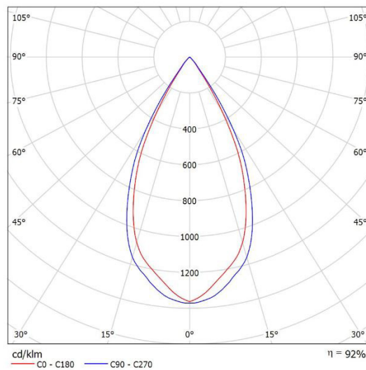
Leuchte: SML L-T6-20T-830-55D Lampen: 1 x CITIZEN-3000K
