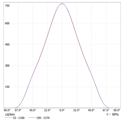
Leuchte: SML_EL-G8R-30T-830D Lampen: 1 x CITIZEN-3000K
