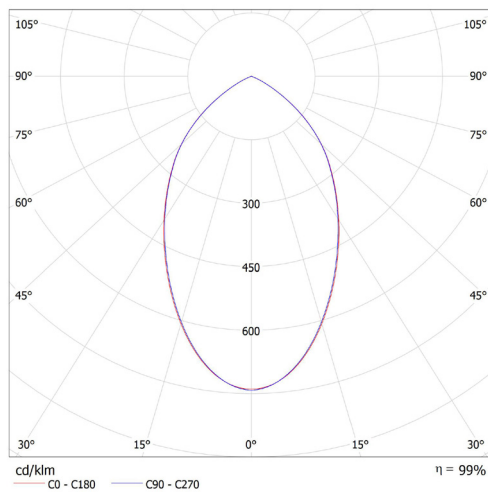
Leuchte: SML_EL-G8R-30T-830D Lampen: 1 x CITIZEN-3000K
