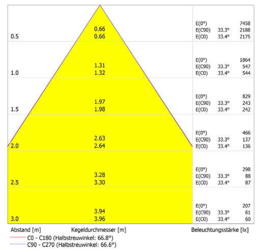
Leuchte: SML EL-G8R-20T-840D Lampen: 1 x CITIZEN-4000K
