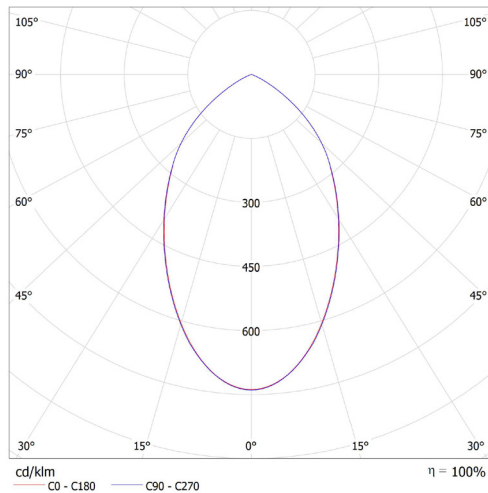
Leuchte: SML_EL-G8R-13T-840D Lampen: 1 x CITIZEN-4000K
