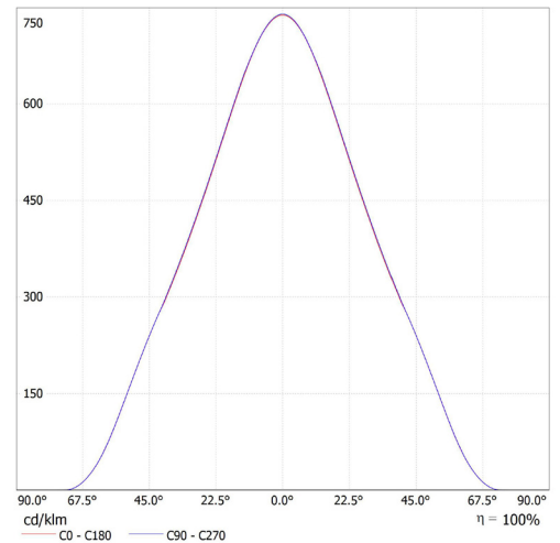
Leuchte: SML_EL-G8R-13T-840D Lampen: 1 x CITIZEN-4000K
