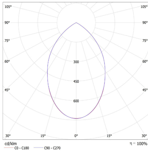
Leuchte: SML EL-G7R-20T-830D Lampen: 1 x CITIZEN-3000K
