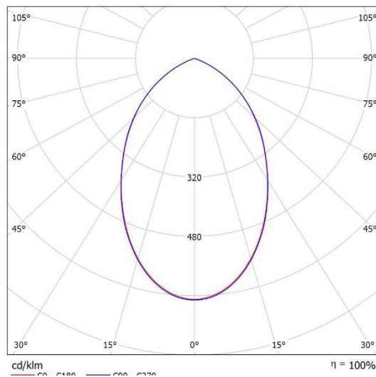
Leuchte: SML EL-G6R-20T-840D Lampen: 1 x CITIZEN-4000K
