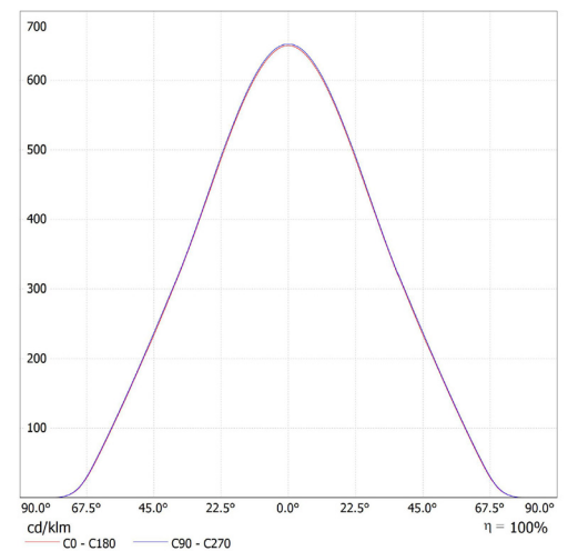
Leuchte: SML EL-G6R-20T-840D Lampen: 1 x CITIZEN-4000K
