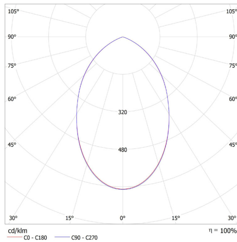
Leuchte: SML EL-G6R-13T-840D Lampen: 1 x CITIZEN-4000K
