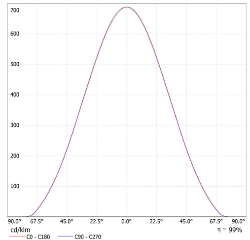
Leuchte: SML EL-G5R-10T-840D Lampen: 1 x CITIZEN-4000K
