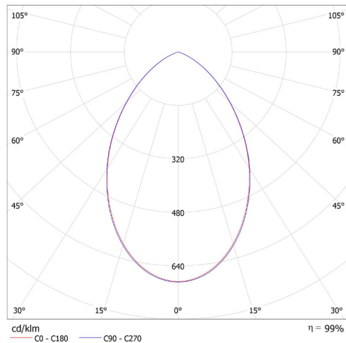
Leuchte: SML EL-G5R-10T-840D Lampen: 1 x CITIZEN-4000K
