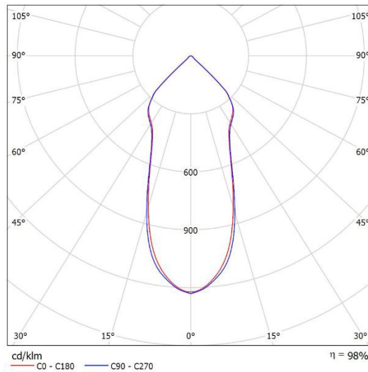
Leuchte: SML EL-E8D-20T-830 Lampen: 1 x CITIZEN-3000K
