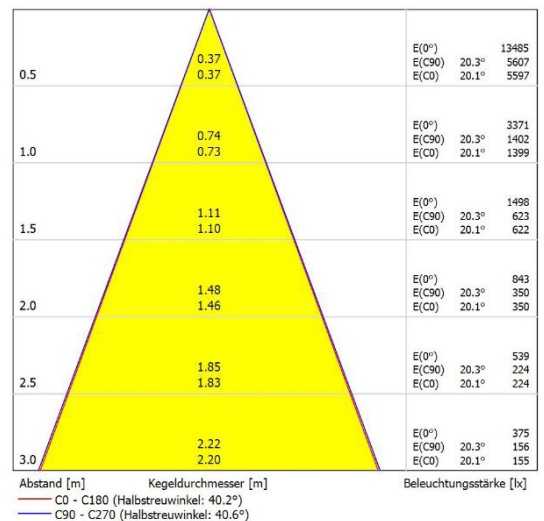
Leuchte: SML EL-E8D-20T-830 Lampen: 1 x CITIZEN-3000K
