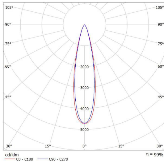
Leuchte: SML_EL-CITA-30T-930-25 Lampen: 1 x CITIZEN-3000K
