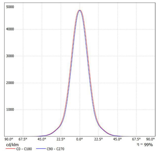
Leuchte: SML_EL-CITA-30T-930-25 Lampen: 1 x CITIZEN-3000K
