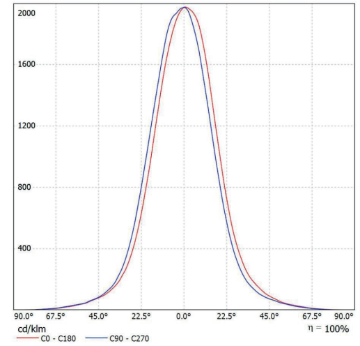
Leuchte: SML KK-DL-65-08-830 Aqua IP65 Lampen: 1 x LED
