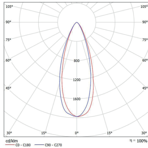
Leuchte: SML KK-DL-65-08-830 Aqua IP65 Lampen: 1 x LED
